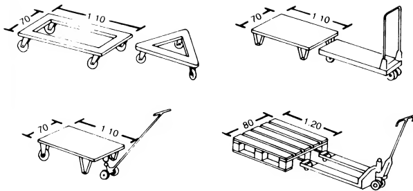
1 Types and dimensions of trolleys used for manual handling in a workshop environment
